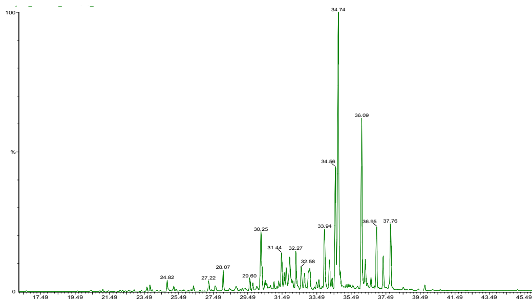
FIG. 1 TYPICAL CHROMATOGRAM OF OIL OF VETIVER (CULTIVATED)
