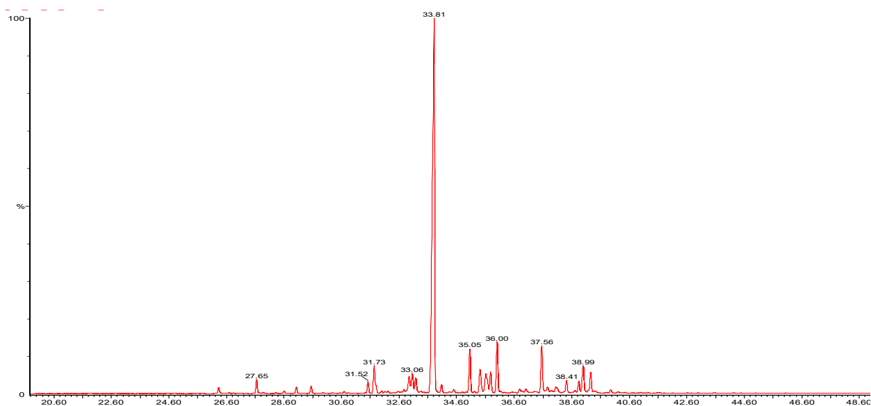
FIG. 2 TYPICAL CHROMATOGRAM OF OIL OF VETIVER (KHUS)
