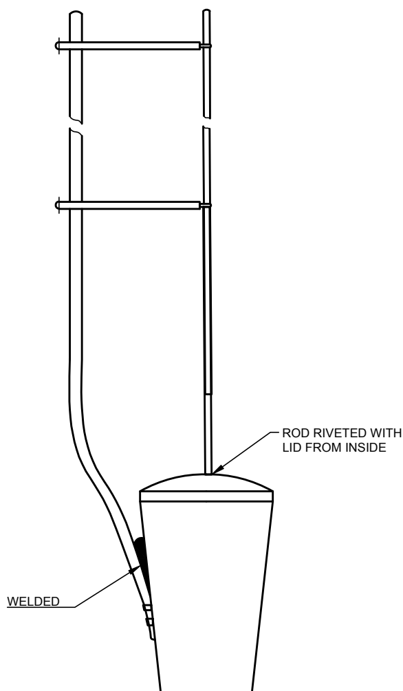
FIG. 1 SAMPLING CAN FOR TANK/TANKER
